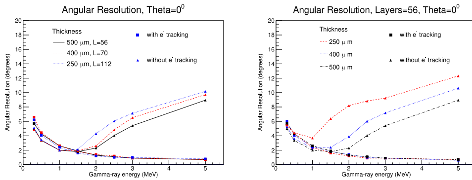
Fig. 2. Angular resolution from the reconstruction of Compton events, Left panel: Fix the radiation length. Right panel: Fix the number of layers.
