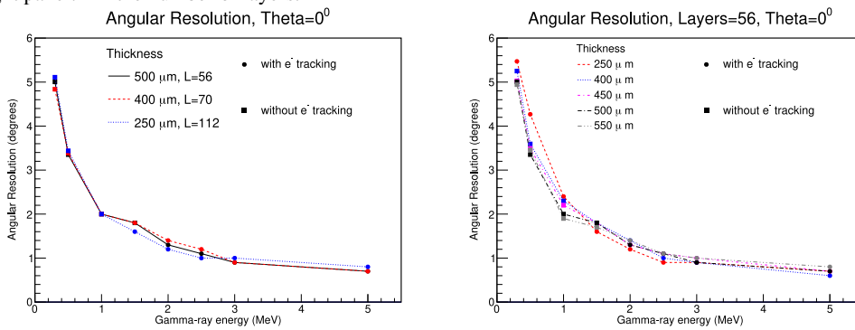
Fig. 3. Angular resolution, after event selection, from the reconstruction of Compton events, Left panel: Fix the radiation length. Right panel: Fix the number of layers.
