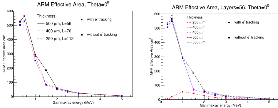
Fig. 4. Effective area from the reconstruction of Compton events, Left panel: Fix the radiation length. Right panel: Fix the number of layers.
