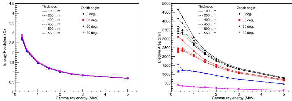
Fig. 5. Energy resolution (left) and Effective area (right) from the photopeak area
